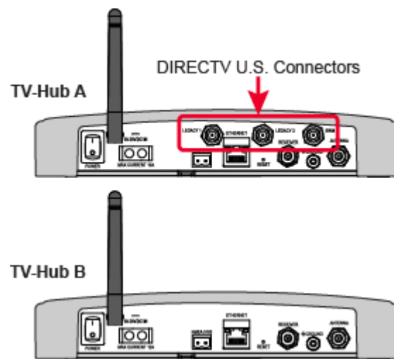
Figure 1-4 TV-Hub Versions
